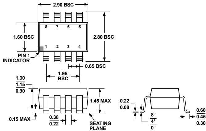
Figure 29. 8-Lead Small Outline Transistor Package [SOT-23] (RJ-8)
